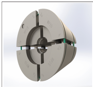
不锈钢夹具 Clamping jaws for stainless steel 1.4571
