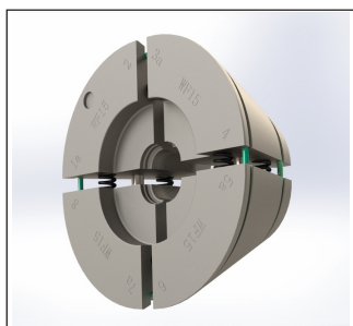
碳钢夹具 Clamping jaws for steel St 37.4/52.4
